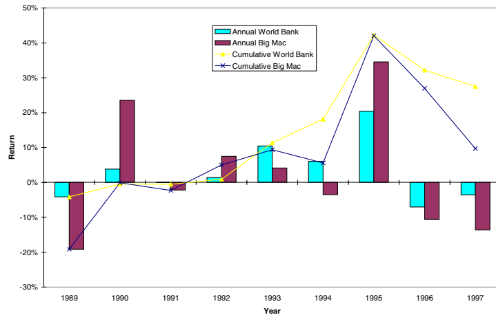
Figure 2 PPP Simulations (1989-1997)
